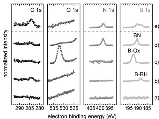
Figure 2. XPS signals of the films. XPS detail spectra (C1s, O1s, N1s, B1s; \text{Al}_{\text{K}\alpha} , h\nu = 1486.6 eV): a) clean Rh(111)/YSZ/Si multilayer substrate; [23] b) CVD of (\text{MeO})_3\text{B} (150 L (\text{MeO})_3\text{B} at 800 K), formation of a Rh-boride phase; c) oxidation of the Rh-boride phase from (b) (925 L \text{O}_2 at 900 K), indicating the presence of B-O(H) species on the surface with a B:O ratio of 1:2; d) addition of ammonia (850 L \text{NH}_3 at 900 K) to the \text{BO}_x phase from (c), formation of BN (ca. 1:1), no oxygen present; e) direct nitrification of a Rh-boride film obtained from CVD of (\text{MeO})_3\text{B} in (b), with 1600 L \text{NH}_3 at 900 K.
